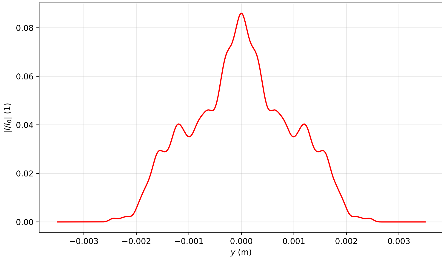
Intensity profile I(x=0, y, z=3.582)/I_0 , \text{Pin}=5.5\text{Pcr} , artificial time
